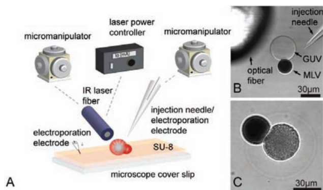
Figure 1. (A) Schematic representation of the components used in the experimental setup. A deposited GUV connected to a multilamellar vesicle (MLV) is shown attached to the SU-8-coated coverslip. (B) Transmission image from the confocal microscope of the optical fiber aligned toward a GUV containing injected polymer solution and connected to an MLV. (C) MLV-GUV with a contracted PNIPAAm-VFc microcompartment, which is centered in the image.
